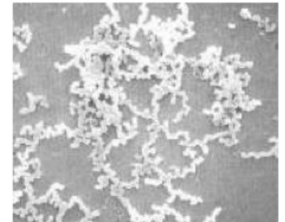
Treated molecules
