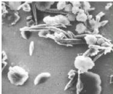
Untreated molecules
